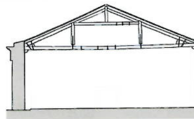
CROSS SECTION C-C'
